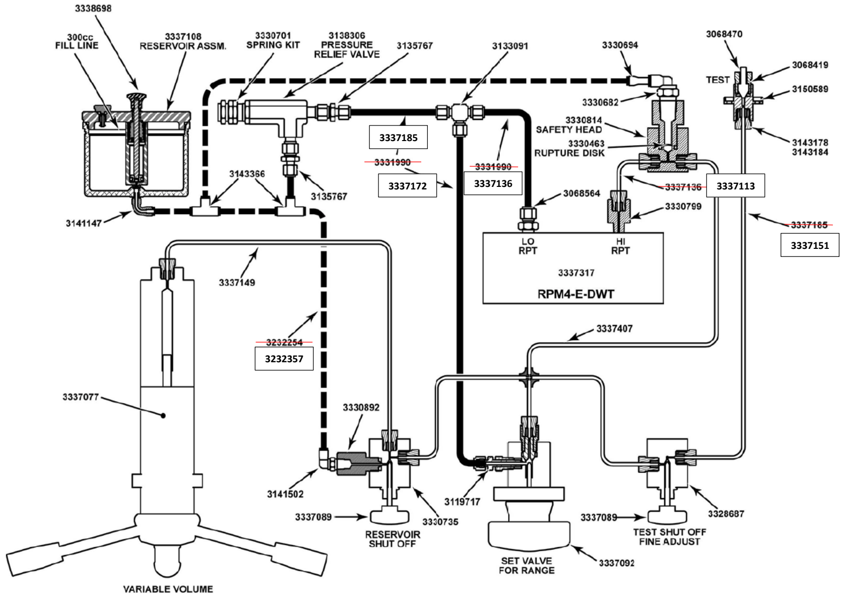
Figure 18. E-DWT detailed hydraulic schematic
