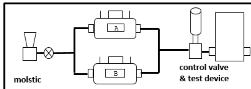
Typical molstic (dual) setup with low pressure or high pressure calibration
